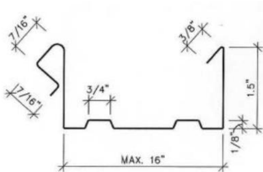
1.5" Snap Lock Panel Dimensions
